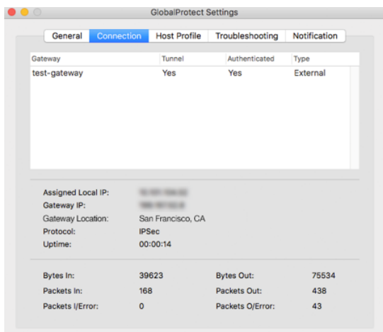
Figure 4: Connection Tab When In External Mode
